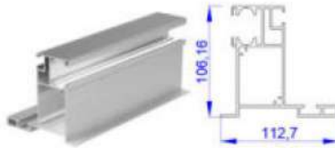
SABİT RAY PROFİLİ FIXED RAIL PROFILE STOK KODU: SG-1015 3,02 KG/ 106,1x112,7x2,2mm
