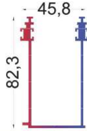
T.2452 - 1,241 KG/MT
