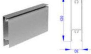
OLUK TAKVİYE PROFİLİ GUTTER REINFORCEMENT STOK KODU: SG-1012 1,82 KG/ 120x30x2mm PROFILE
