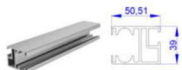
HAREKETLİ RAY PROFİLİ TELESCOPIC RAIL PROFILE STOK KODU: SG-1016 1,28 KG/ 39x50,5x2,2mm
