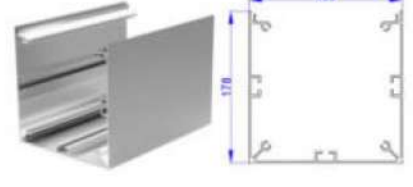
DİREK PROFİLİ COLUMN PROFILE STOK KODU: SG-1013 5,00 KG/ 178x180x2,3mm
