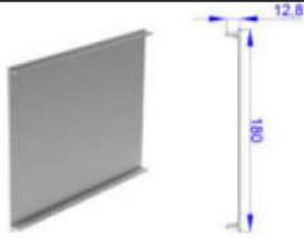
DİREK KAPAK PROFİLİ COLUMN CAP PROFILE STOK KODU: SG-1014 1,11 KG/ 180x12,8x2mm
