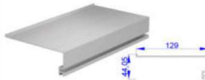
TAKVİYE KAPAMA PROFİLİ STOK KODU: SG-1024 REINFORCEMENT CAPPING PROFILE 0,93KG/ 44,05x129x1,6mm
