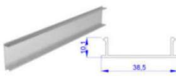
LED KAPAĞI PROFİLİ LED COVER PROFILE STOK KODU: SG-1018 0,16 KG/ 10,1x38,5x1mm
