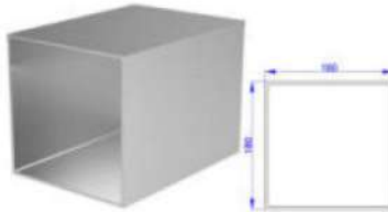
DİKME KUTU PROFİLİ UPRIGHT BOX PROFILE STOK KODU: SG-1021 7,65 KG/ 180x180x4mm
