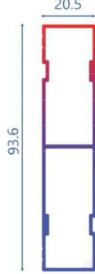
T.2353 0.968 KG/MT 3 KANALLI YAN KASA
