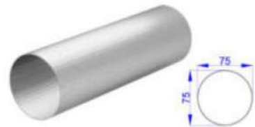
SU TAHLİYE PROFİLİ DRAINAGE PROFILE STOK KODU: SG-1022 1,24 KG/ 75x75x2mm
