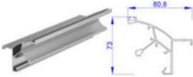
LED PROFİLİ LED PROFILE STOK KODU: SG-1017 1,21 KG/ 73x80,8x1,8mm
