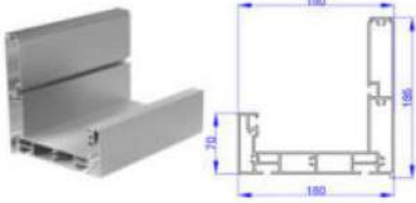
OLUK PROFİLİ GUTTER PROFILE STOK KODU: SG-1011 6,36 KG/ 185x180x2,2mm
